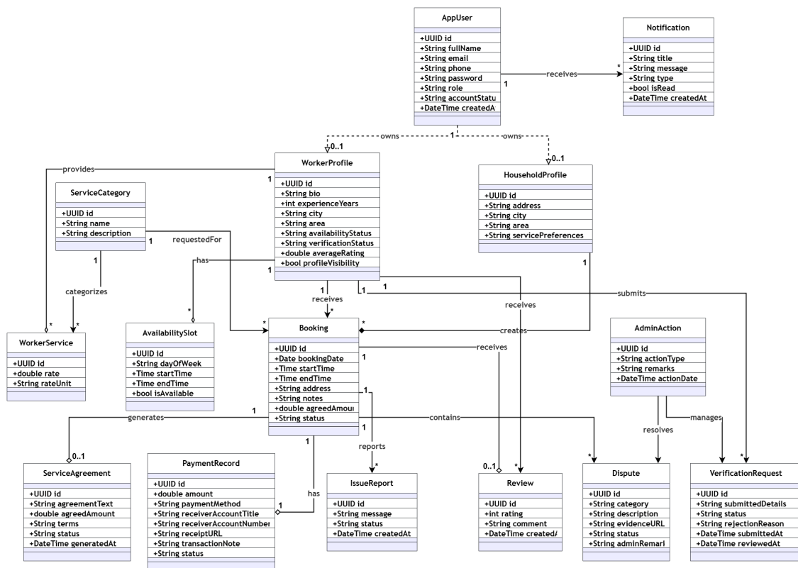
Figure 4.3 Class Diagram of HomeEase Core Domain Models
